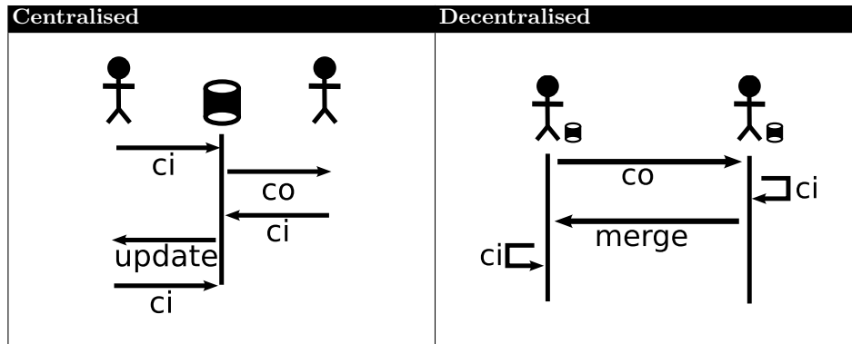
Fig. 1. A graphical depiction of the typical cooperation of two developers using both a centralised and a decentralised source and configuration management system. We use the common mnemonics co and ci to denote check-out and check-in respectively.
